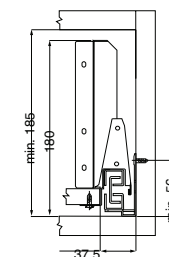
Cabinet drilling dimensions
