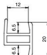
Linear junction
