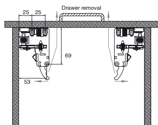
Bottom view of drawer
