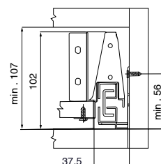
Cabinet drilling dimensions
