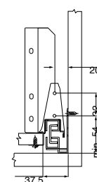
Front drilling dimensions
