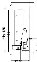
Cabinet drilling dimensions
