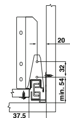
Front drilling dimensions
