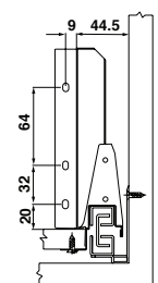
Back drilling dimensions
