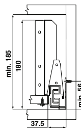
Cabinet drilling dimensions
